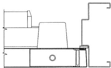
LOCK STILE SINGLE DOOR
