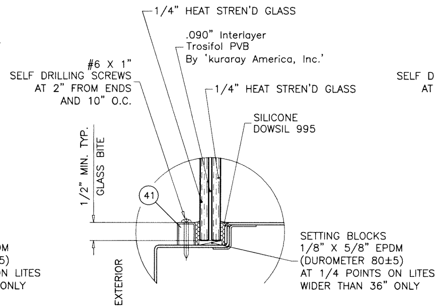
GLASS TYPE 'B'
