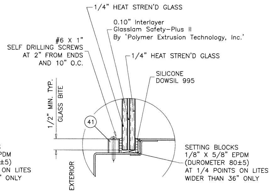
GLASS TYPE 'B1'
