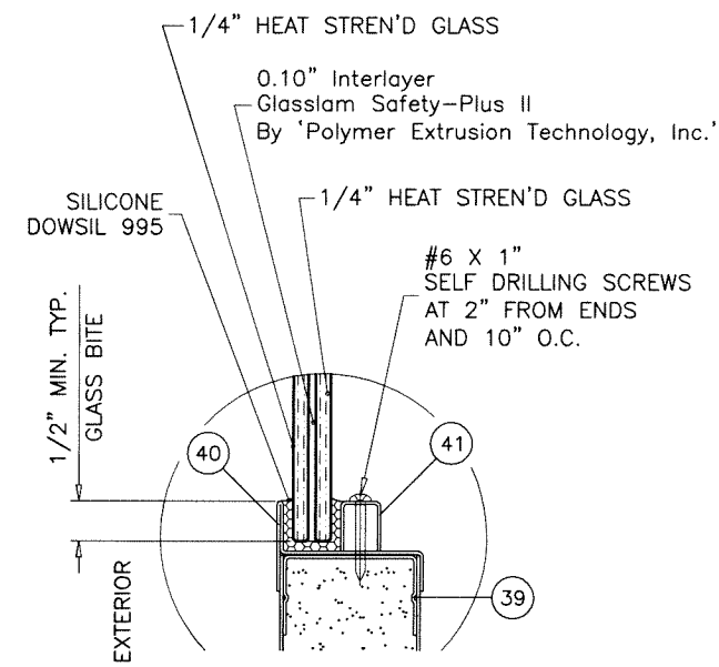
GLASS TYPE 'B1'
