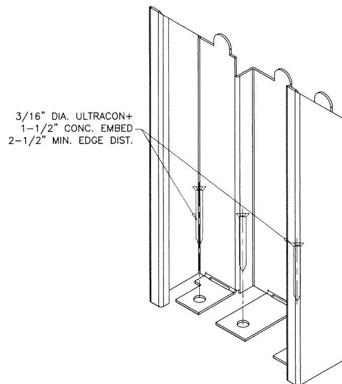
DOUBLE RABBET FLOOR ANCHOR DETAIL OPTIONAL
