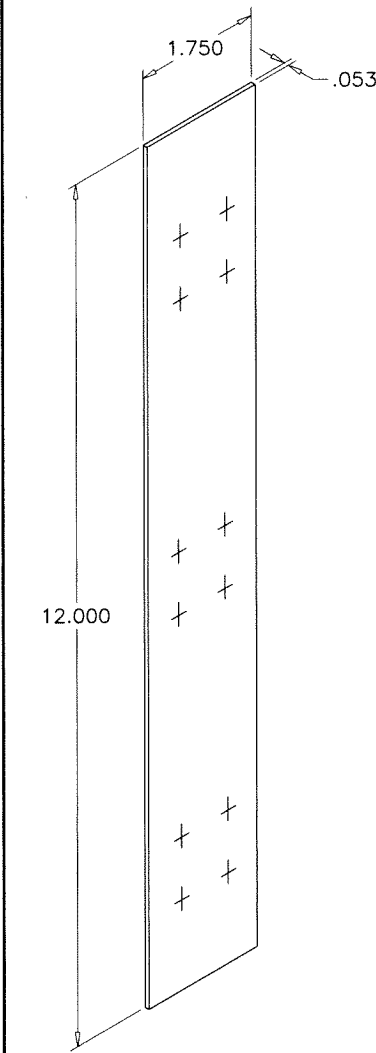
10 REINF. PLATE
