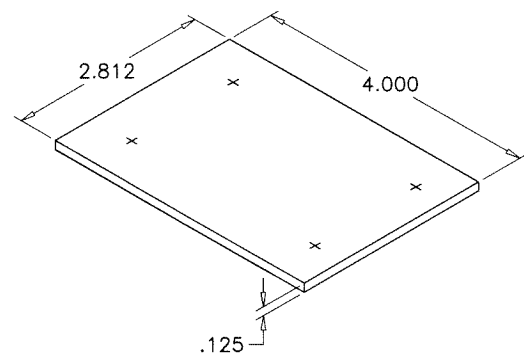
6 REINF. PLATE
