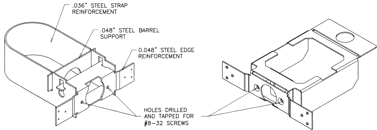
31 CYLINDRICAL LOCK & DEAD BOLT REINF.
