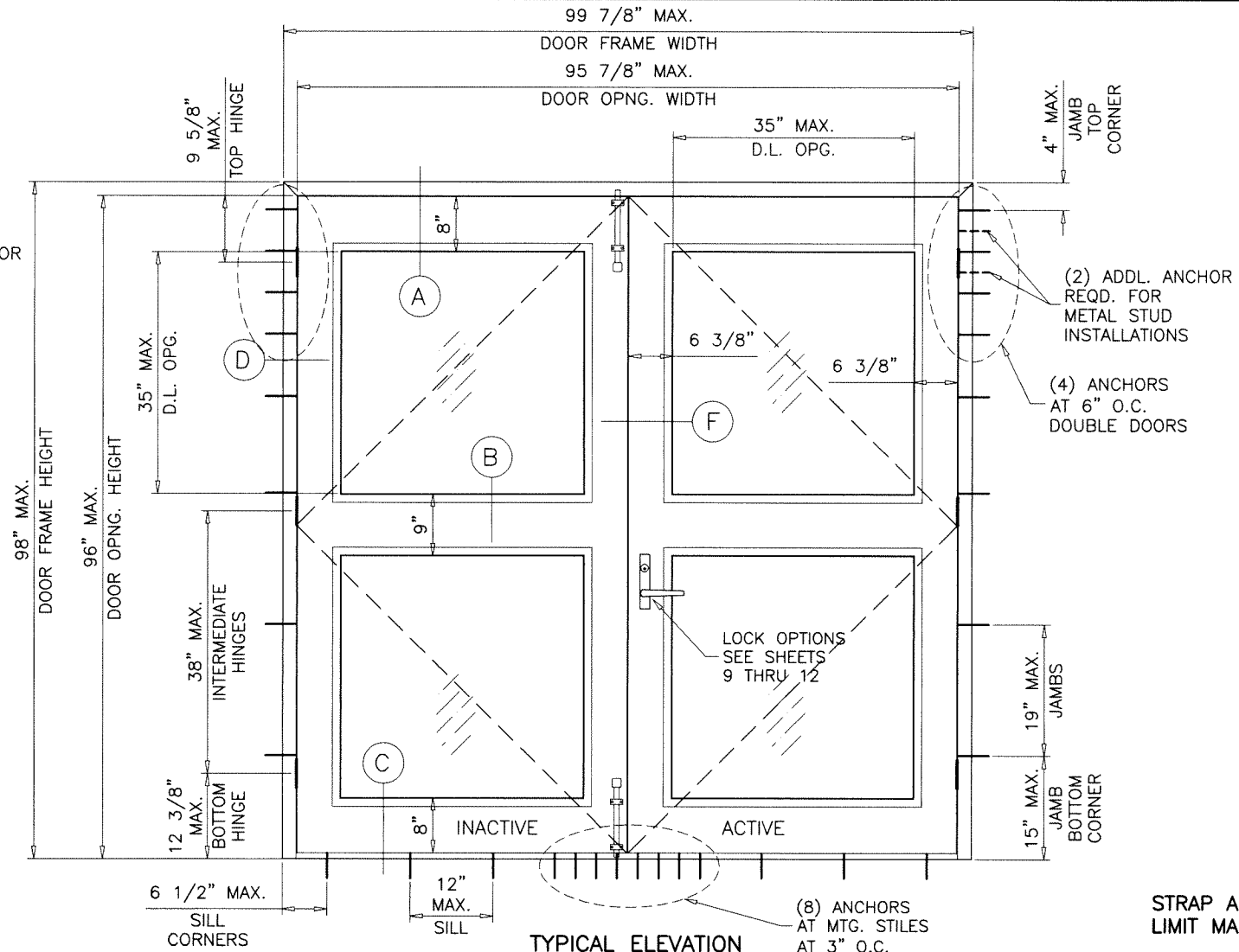
TYPICAL ELEVATION
