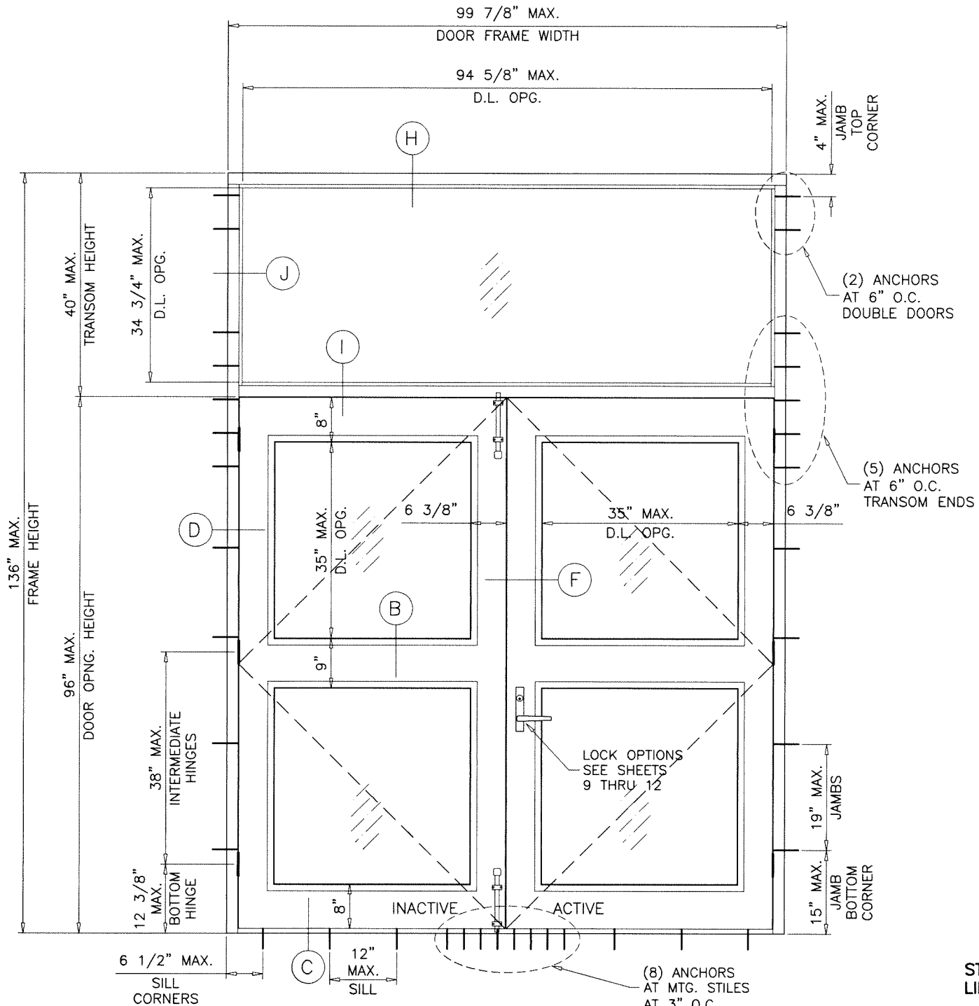
TYPICAL ELEVATION ( O/XX )
