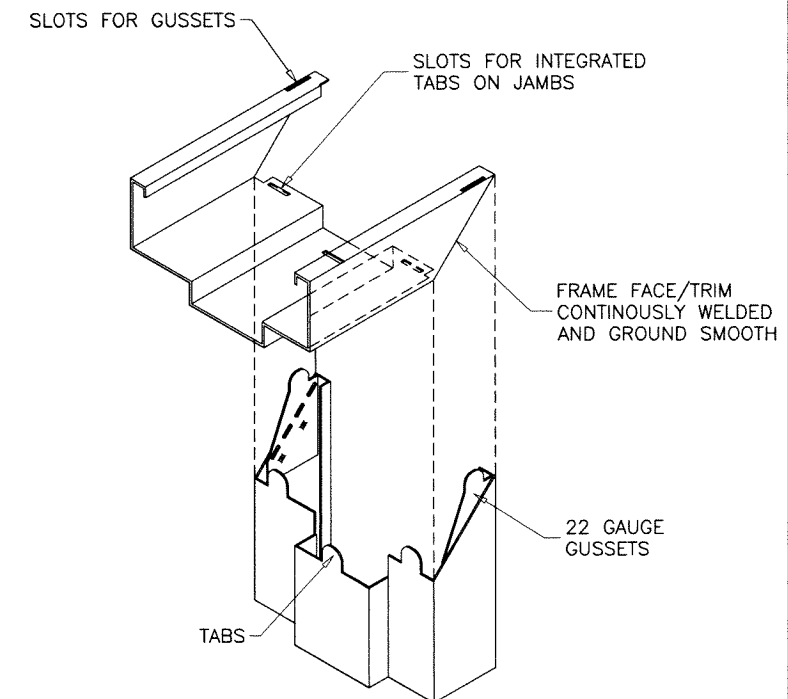
FRAME CORNERS OPTION #2
