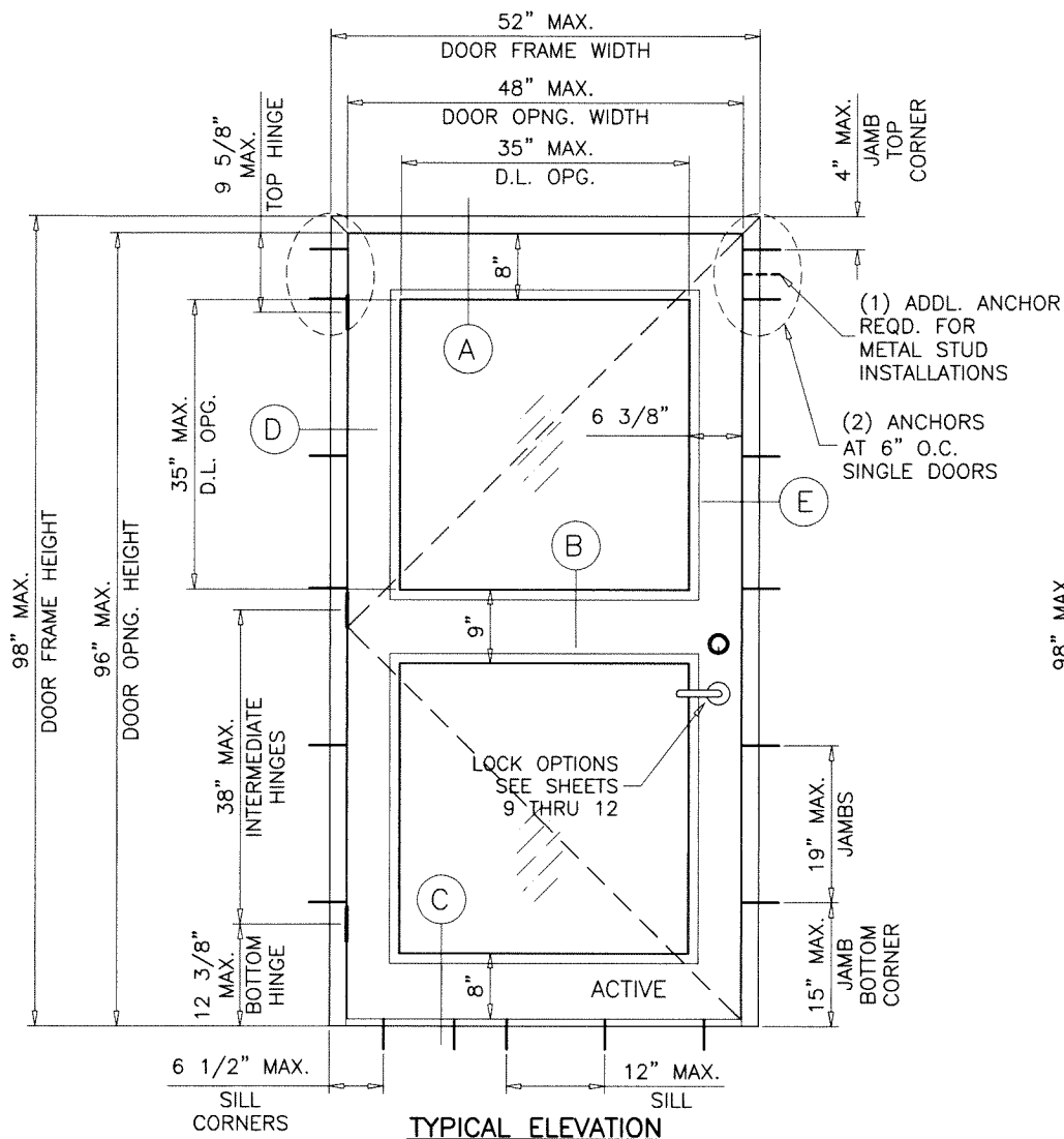
TYPICAL ELEVATION
