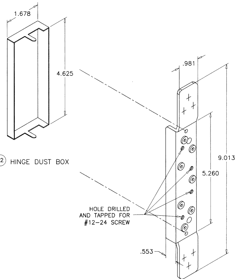
13 HINGE REINF.
