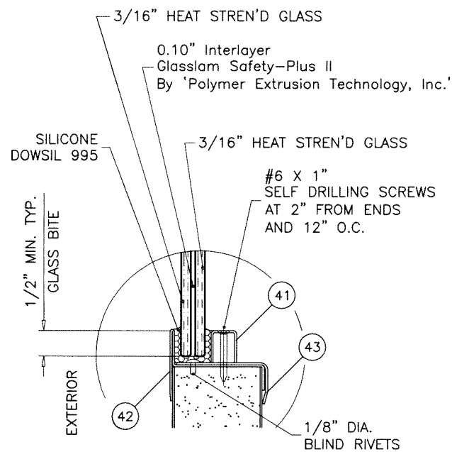
GLASS TYPE 'A' 7/16" LAM. GLASS
