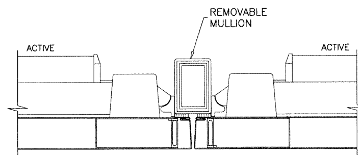
MTG. STILES DOUBLE DOOR WITH MULLION
