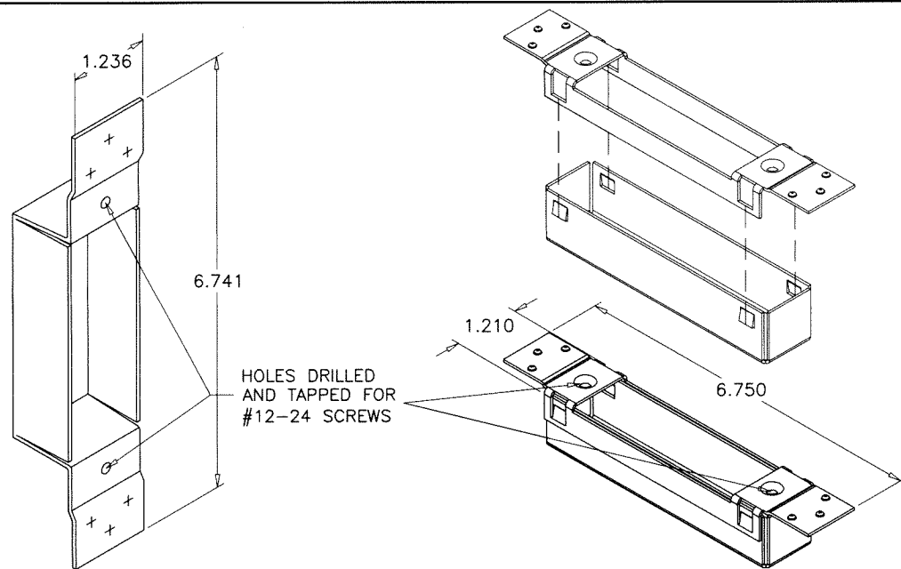
15 ASA STRIKE BOX
