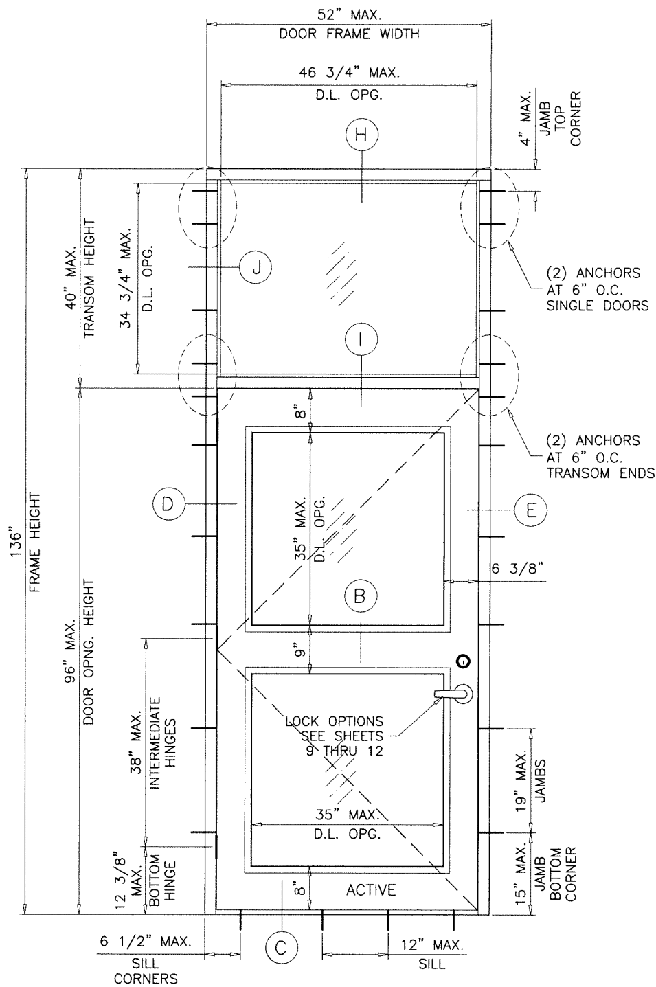
TYPICAL ELEVATION ( O/X )
