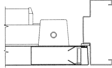
LOCK STILE SINGLE DOOR
