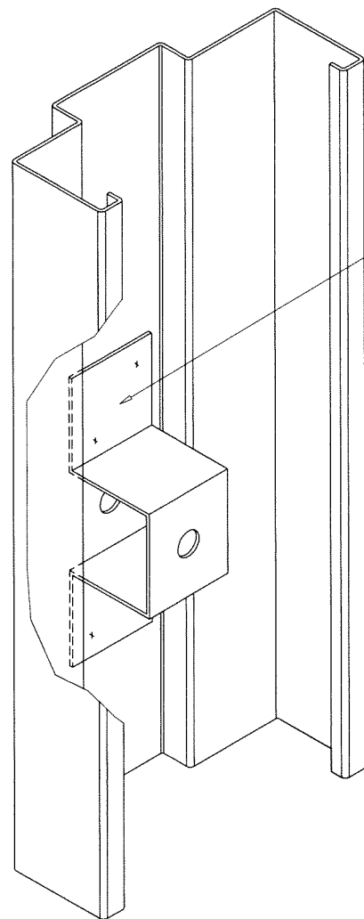
FRAMES WITHOUT GROUT OPTION
