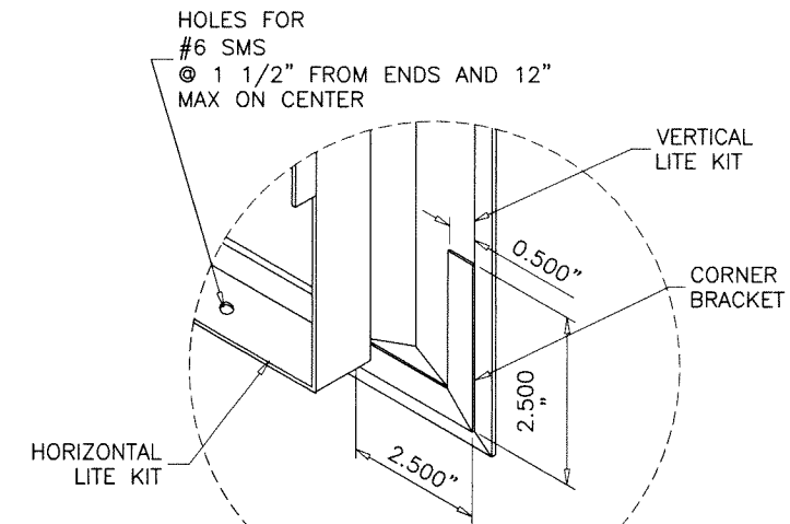
DETAIL 'A' CORNER BRACKET DETAIL
